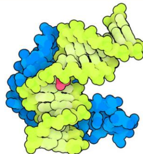
Cisplatin and DNA
