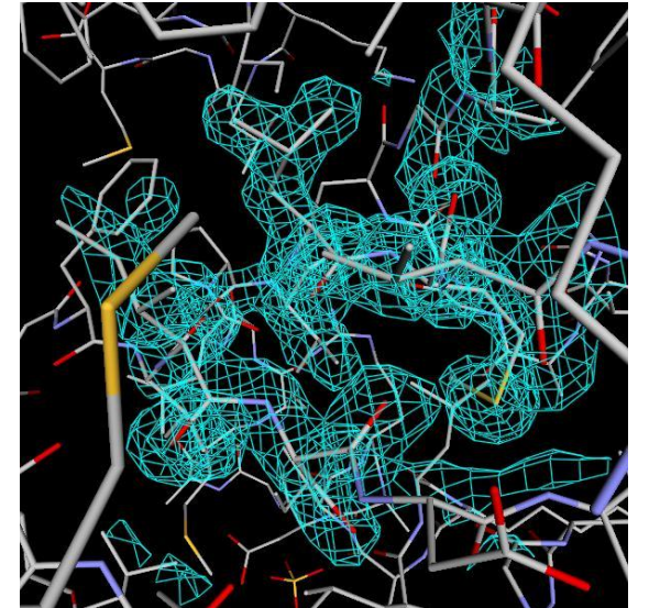
Electron density
