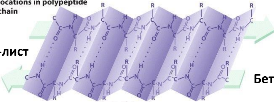
Pleated sheet
