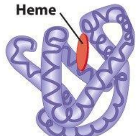
β polypeptide
