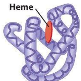
β polypeptide
