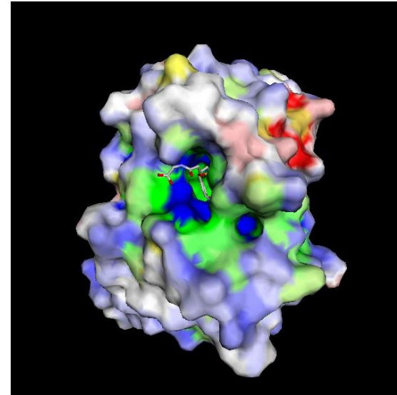
Molecular surface
