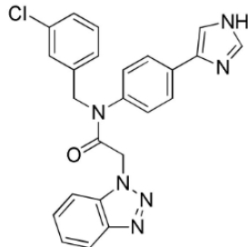
2 Benzotriazole CCF981
