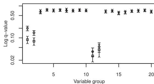
Fig. 2. Distribution of enrichment FDR for simulated variable groups using both unoptimized and optimized annotations. Plotted FDR values were computed using the Benjamini and Hochberg algorithm from two-sided enrichment P -values generated by the competitive enrichment method CAMERA (Wu and Smyth, 2012) for each of the 20 variable groups across 25 datasets simulated according to the design outlined in Section 2.3.1. Filled circles and flat error bars represent the average ( \pm one standard error) of the FDR values computed for each of the 20 variable groups using unoptimized annotations on the 25 simulated datasets. Squares and angled error bars represent the FDR values computed using bootstrap optimized annotations with strict filtering. For the four enriched variable groups simulated with a true mean difference between cases and controls, open circles and open squares are used. FDR values are plotted on a logarithmic scale
