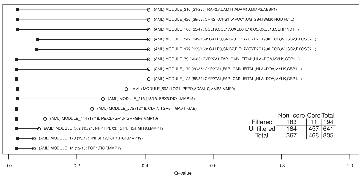
Fig. 4. Enrichment and annotation optimization results for the MSigDB C4 v4.0 cancer modules and leukemia gene expression data (Armstrong et al. , 2002). The figure shows the difference between enrichment FDR computed using unoptimized and optimized annotations for the 15 cancer modules with the lowest unoptimized enrichment P -values. Enrichment FDRs were computed using the Benjamini and Hochberg algorithm on two-sided P -values generated by CAMERA (Wu and Smyth, 2012). Open circles represent the FDR values computed using the unoptimized cancer module annotations, and solid squares represent the FDR values computed using optimized cancer modules. If the optimized FDR value is less than the unoptimized value, a solid line is used, otherwise, a dotted line is used. An AML prefix is used for gene sets enriched using the unoptimized annotations for the acute myeloid leukemia, and an ALL prefix is used for gene sets enriched for the acute lymphoblastic leukemia phenotype. The ratio of optimized to unoptimized annotations for each of the top 15 cancer modules is displayed after each module name along with the symbols for the filtered genes (cropped at 7). An asterisk follows the symbol for filtered annotations that were designated as core genes by the GSEA algorithm. For the displayed contingency table, filtered annotations were removed by EMVC in more 85% of the cluster results in 50 bootstrap resampled data sets resulting in an odds ratio of 41.1 (95% CI: 21.8–86). When all filtering thresholds are considered, the area under the ROC curve is 0.92
