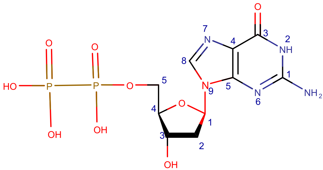
2'-deoxyguanosinediphosphate
