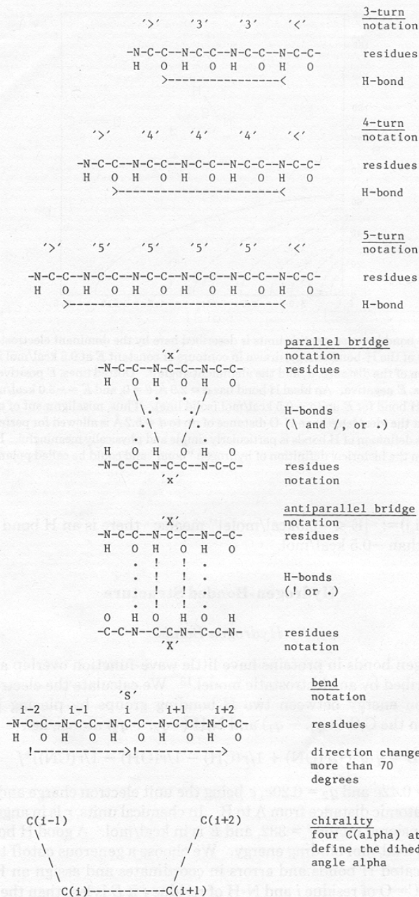
Fig. 2. Elementary patterns used in structure definition.
