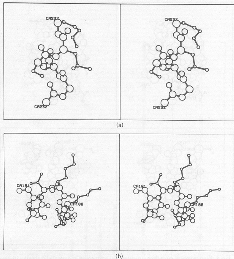
Fig. 3. Stereoviews of secondary structure: (a) 3-helix ( 3_{10} -helix) and (b) 5-helix ( \pi -helix). (a) 3-Helix Gly232-Lys237 from triose phosphate isomerase (TIM). In Table AIII, it appears as the H-bond pattern
