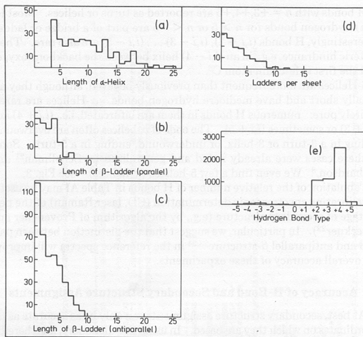
Fig. 6. The common feature of the size distribution of secondary structure segments is the gradual fall-off: larger sizes are less probable than smaller ones. Note that we give (b,c) the length of \beta -ladders (strand pairs) rather than the length of \beta -strands. A strand is often longer than the ladders in which it participates, since sheets tend to be trapezoidal rather than rectangular in shape. The number of bulge-linked ladders per sheet (d) is given as an indication of the width of the sheet. The width of a ladder is about 5 Å. In an ideal sheet, center strands take part in two ladders, edge strands in one: the number of ladders is equal to the number of strands minus one. In general, however, one strand can participate in more than one ladder on each side and the width of the sheet less than the number of ladders times 5 Å. Note: sheets consisting of a single bridge are not included in the histogram of ladders per sheet. (e) Number of H-bonds of type (CO(i), NH(i+n)) . Due to the nature of L-amino acids, positive n are heavily favored. The dominant peak at n = 4 represents \alpha -helices and 4-turns. We find that H bonds (i, i+2) and (i, i+3) are surprisingly common, though generally weak.
