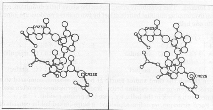
Fig. 5. Stereoviews of secondary structure: illustration of chirality. This short left-handed \alpha -helix, Gln225-Val230 from thermolysin (2TLN) is the only one known to us. In Table AIII (note that chirality is entered at the second residue of each quartet) it appears as:
